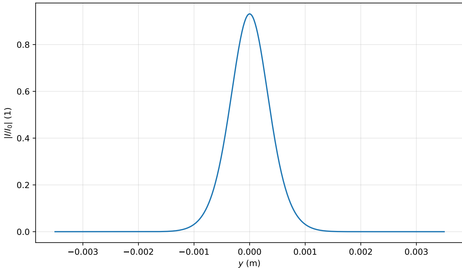
Intensity profile I(x=0, y, z=1.274)/I_0 , P_{in}=0.4P_{cr} , artificial time
